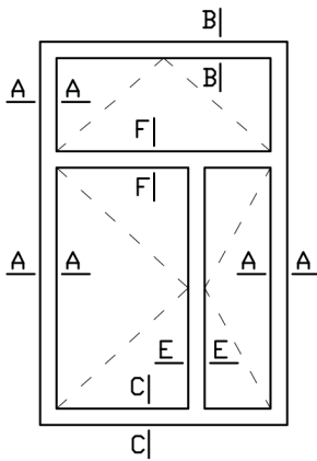
Folding double-hung window, fixed post
