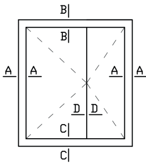
Folding single-hung window, movable post
